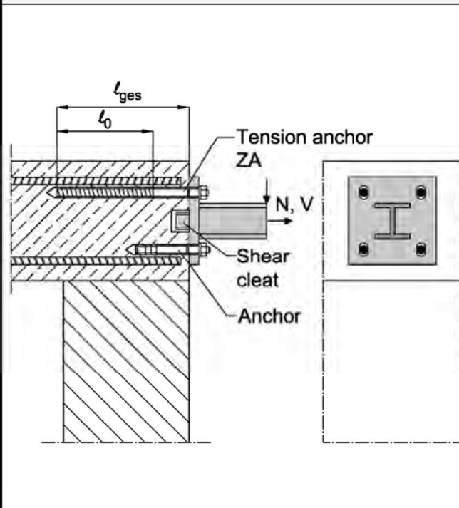
Figure A8: Overlap joint for the anchorage of cantilevers
